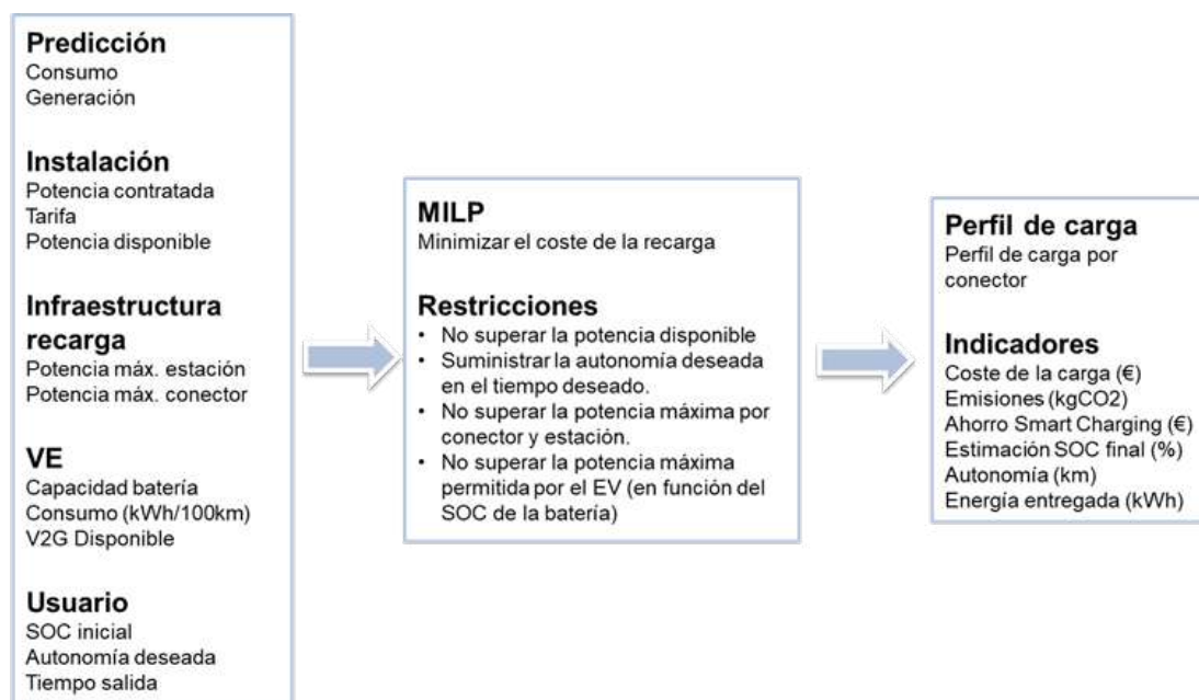
Diagrama conceptual de SmartCharging.
